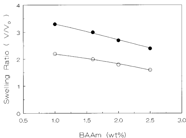
Figure 3 Variation of the equilibrium swelling ratio of PNIPA gels, V/V_0 , with the crosslinker (BAAM) content. Swelling measurements were performed at (●) 4^\circ\text{C} and (○) 23^\circ\text{C} \pm 1 . The gel preparation temperature: 25^\circ\text{C} .
