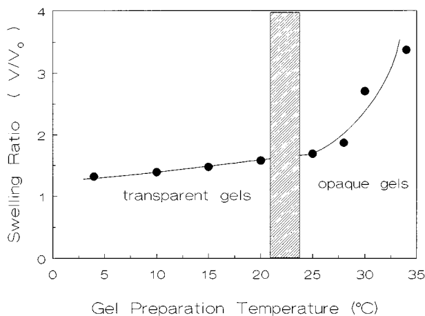
Figure 2 Variation of the equilibrium swelling ratio of the PNIPA gels, V/V_0 , with the polymerization temperature. BAAM: 2 wt %. Swelling temperature: 23^\circ\text{C} \pm 1 . The shaded area represents the transition region from homogeneous to heterogeneous gels.
