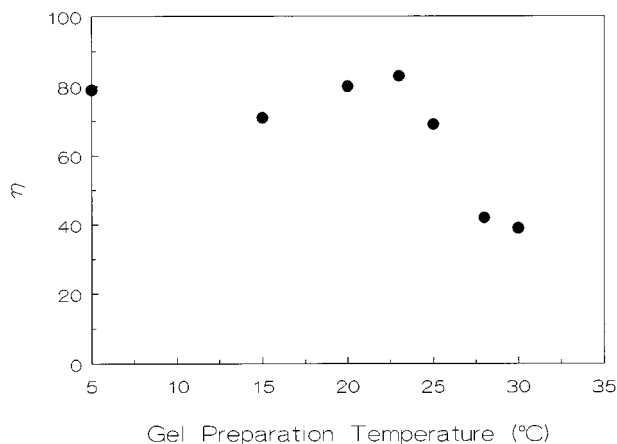
Figure 7 Variation of the separation efficiency \eta of PGA with the gel preparation temperature. Swelling experiments were performed at 4^{\circ}\text{C} . BAAm content of the PNIPA gel: 2 wt %.
